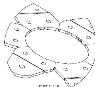
DETAIL B SCALE 1 : 5
